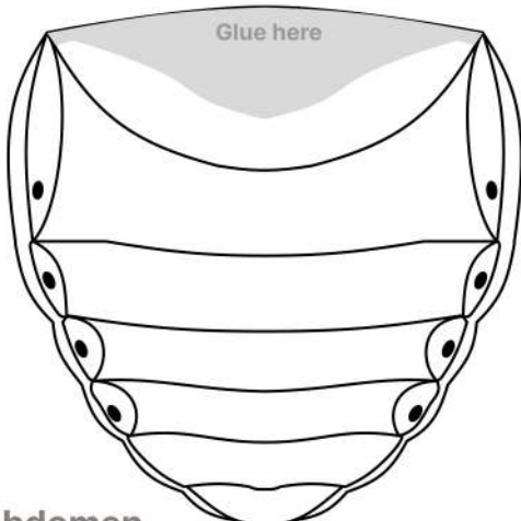
Abdomen
